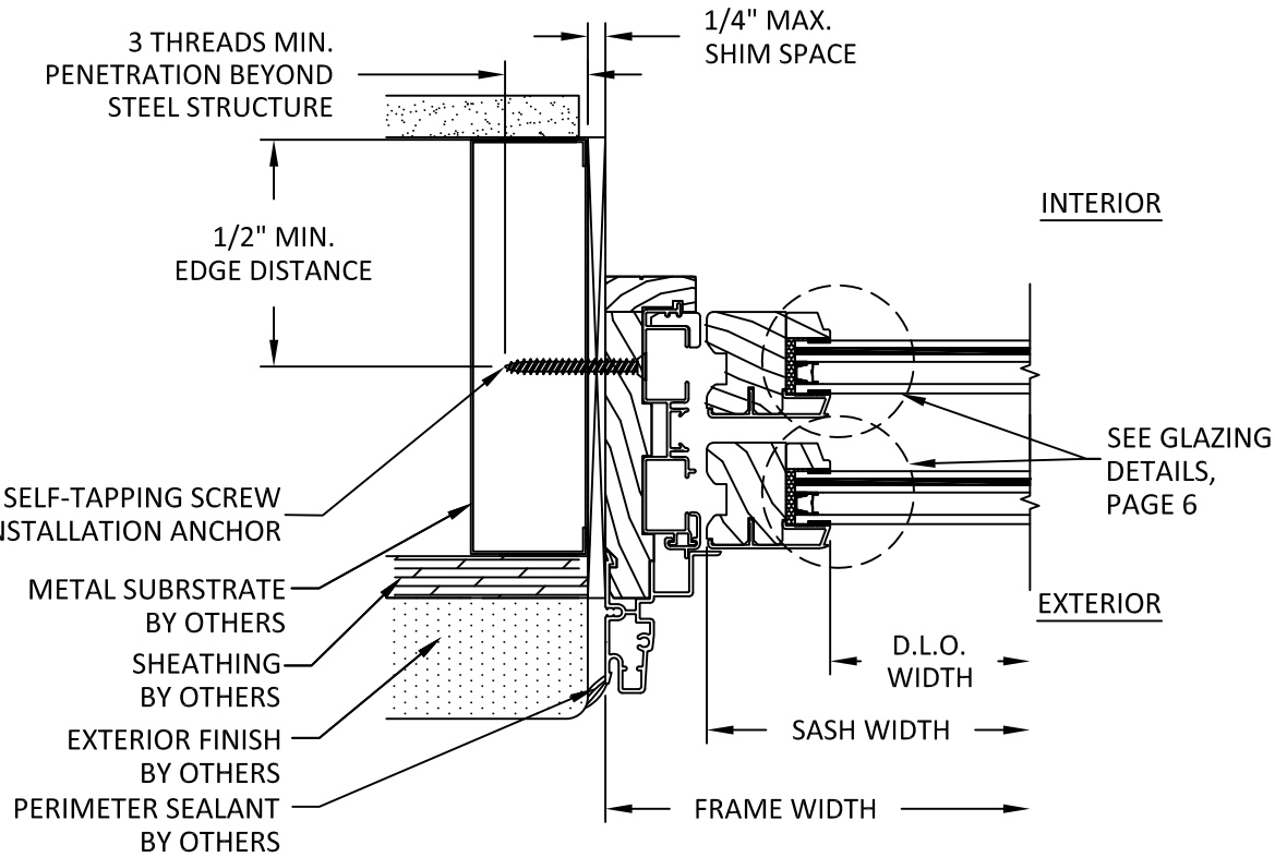
C 3 HORIZONTAL SECTION DH JAMB - STEEL STUD FRAME THROUGH FRAME INSTALLATION
