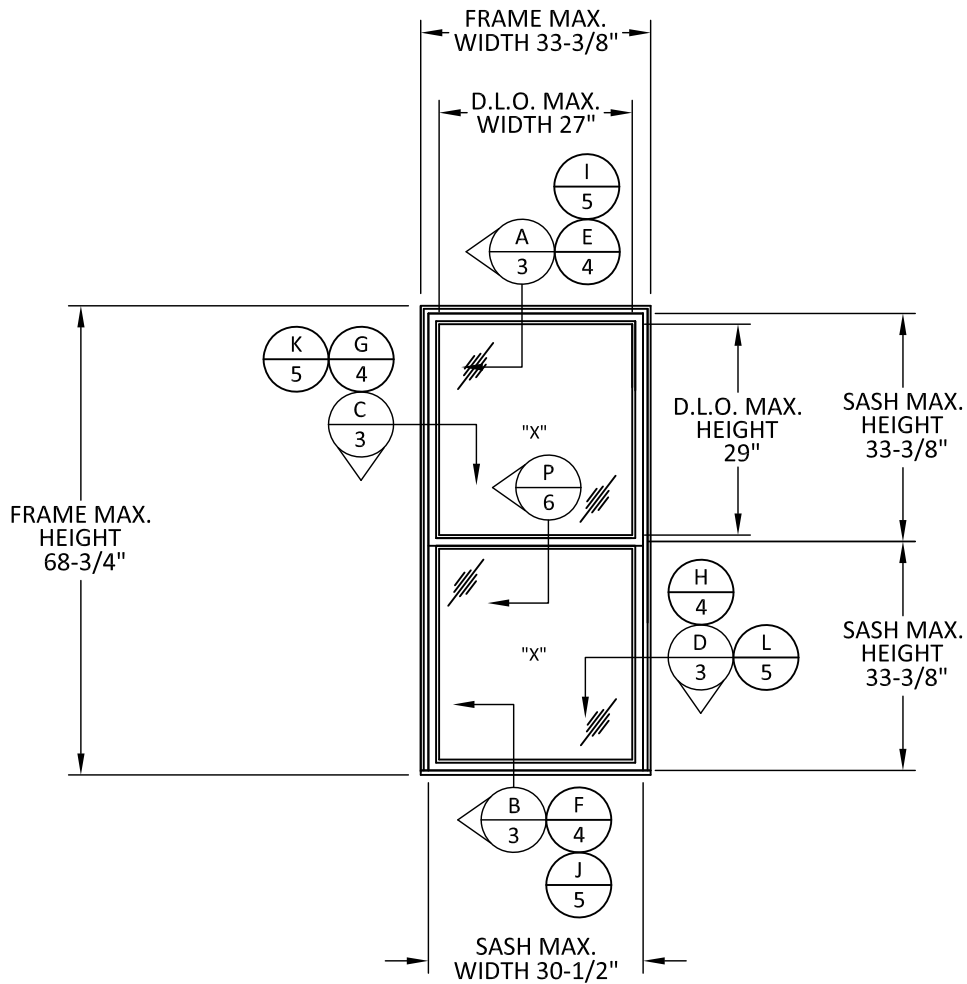
TYPICAL ELEVATION DOUBLE HUNG
