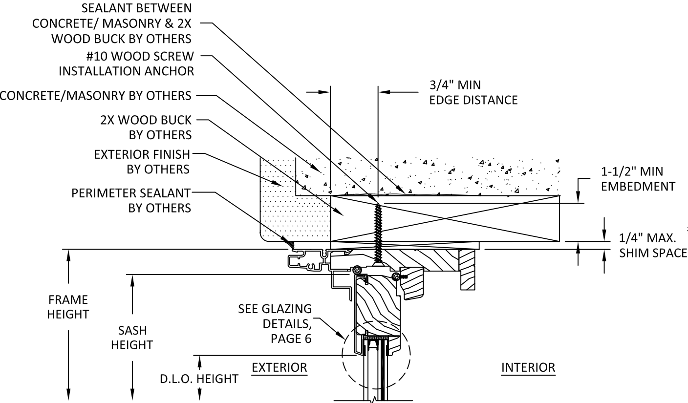
A 3 VERTICAL SECTION DH HEAD - 2X WOOD BUCK THROUGH FRAME INSTALLATION
