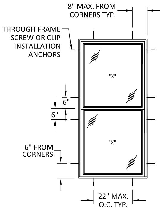
ANCHOR LAYOUT CLIP OR SCREW INSTALLATION
