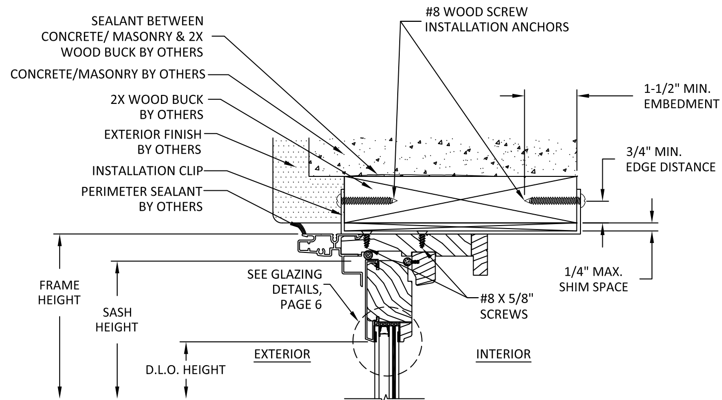
E 4 VERTICAL SECTION DH HEAD - 2X WOOD BUCK STANDARD CLIP INSTALLATION
